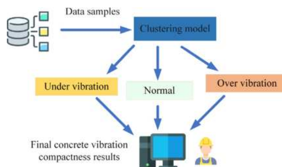
Fig. 19. Prediction model.
